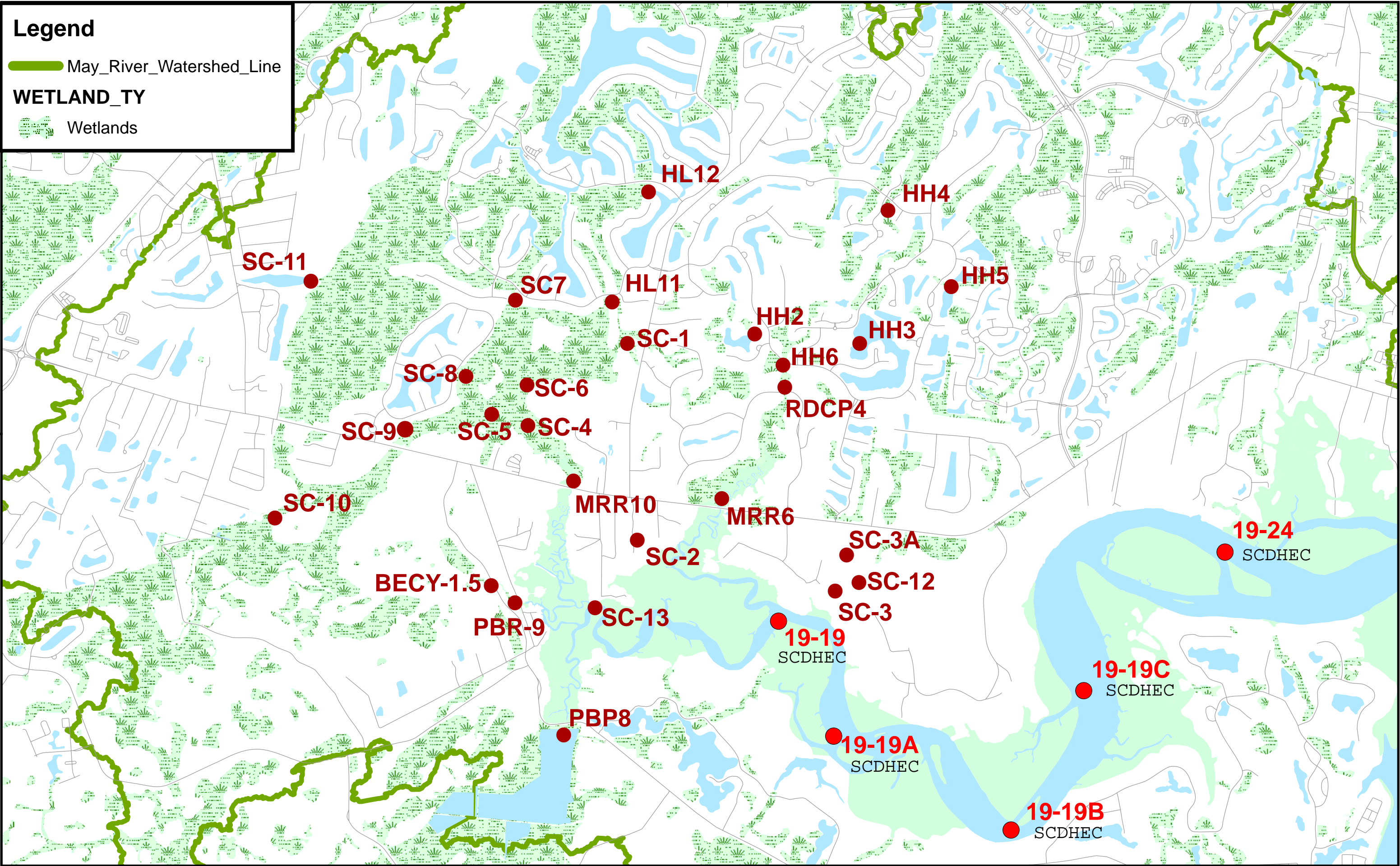
SCDHEC Shellfish & Weekly Sampling Sites within Stoney and Rose Dhu Creek Subdrainage Basins
